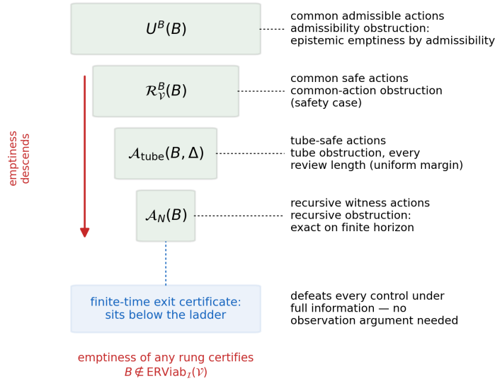
Figure 1: The obstruction ladder. The common response sets form nested necessary conditions for viability, U^B(B) \supseteq \mathcal{R}_{\mathcal{V}}^B(B) \supseteq \mathcal{A}_{\text{tube}}(B, \Delta) \supseteq \mathcal{A}_N(B) , and emptiness descends (Proposition 2); the finite-time exit certificate sits below the ladder, defeating every control under full information (Theorem 4).
